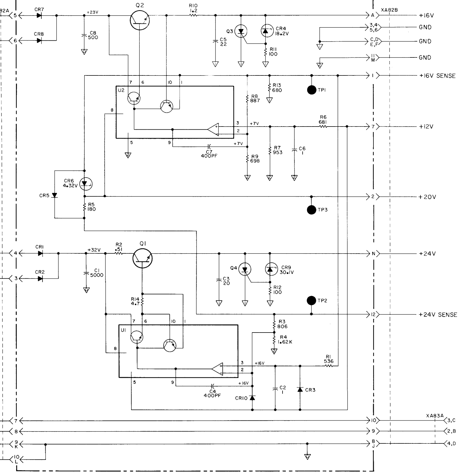
+16V and +24V POWER SUPPLY ASSEMBLY A82
