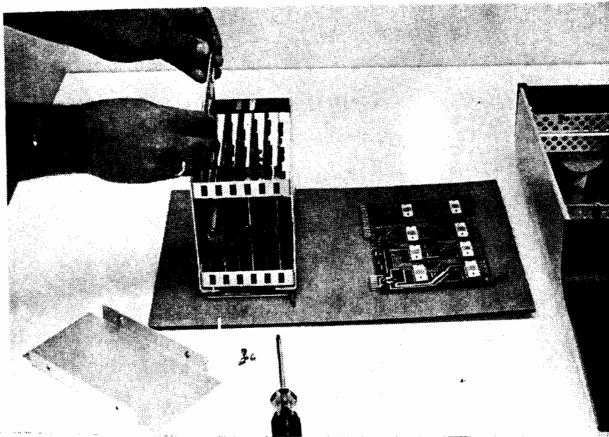
Figure 2-11. Exchanging PC Boards in the Memory Assembly
