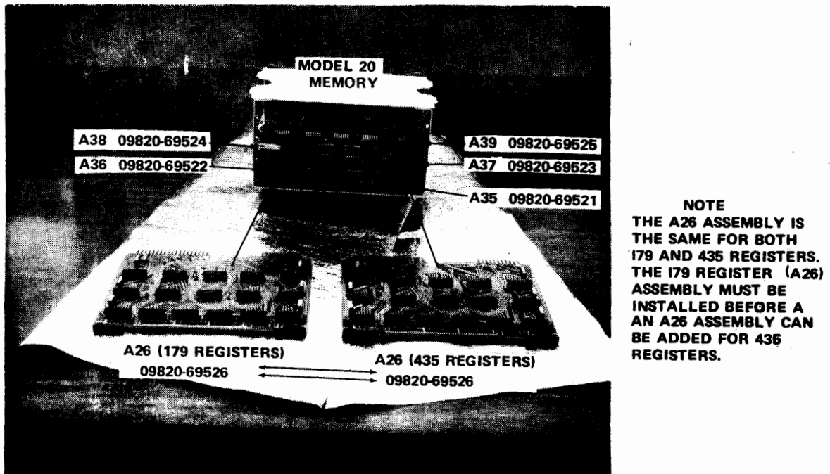
Figure 2-10. The 9820A Memory Configurations.
