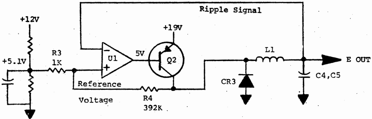
Figure 6-3. +5V Simplified Schematic
