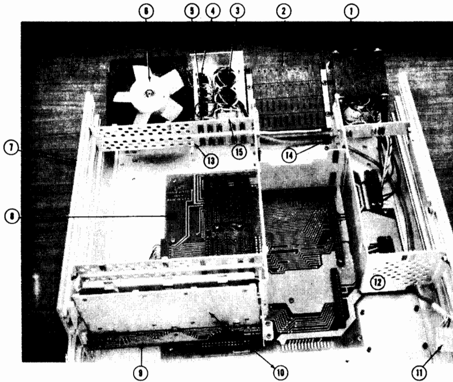
Figure 6-11. 9810A and 9820A Back Panel and Chassis Parts
