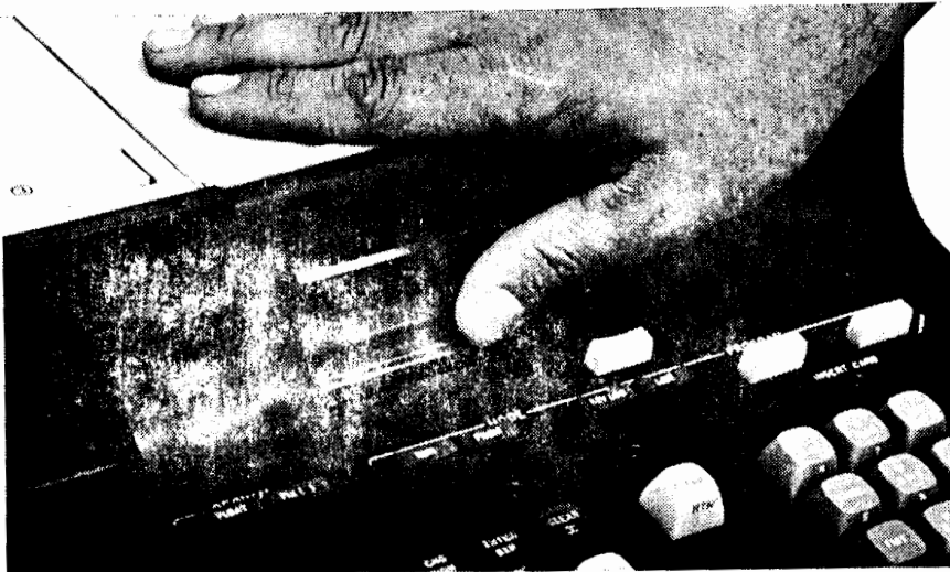
Figure 2-5. Installing the Printer Window
