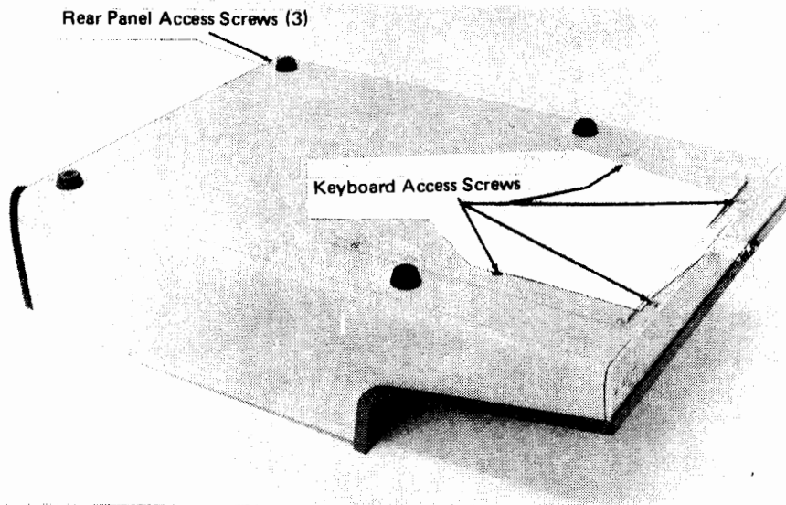
Figure 5-4. The Keyboard Access Screws
