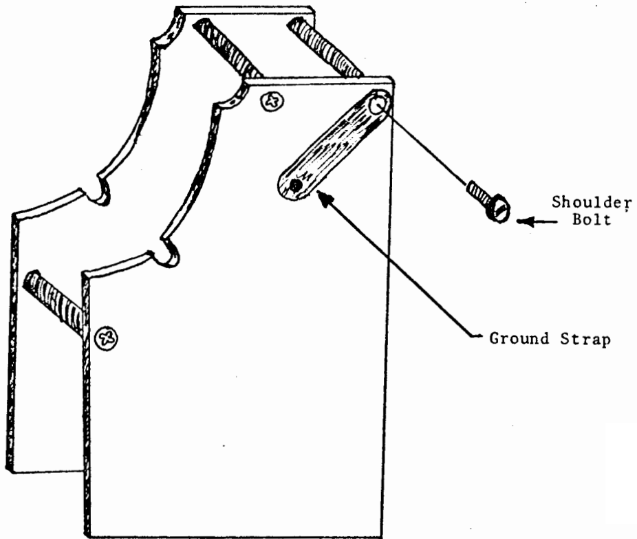
Figure 13. Ground Strap Installation
