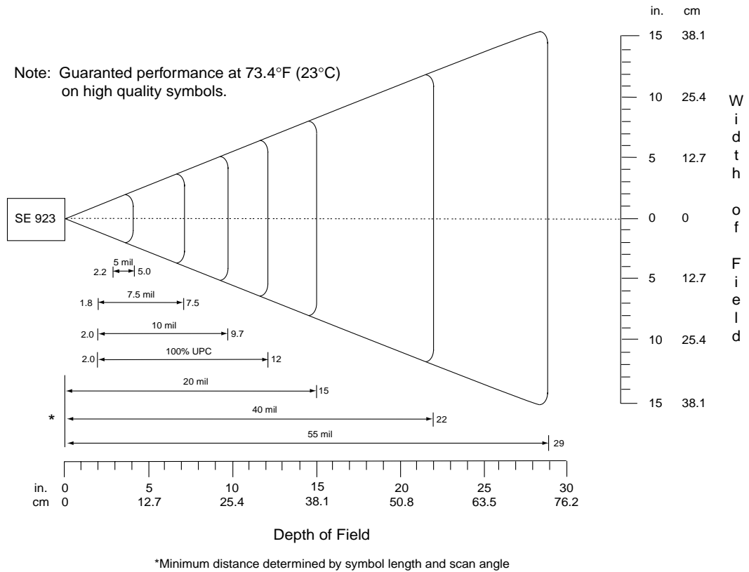
Figure 3-2. SE-923-I000A Standard Version Decode Zone
