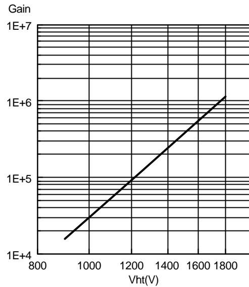
Typical gain curve
